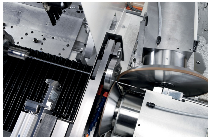
Example of pinch/peel grinding of a long and thin component on the Rollomatic ShapeSmart® NP50 grinding machine
